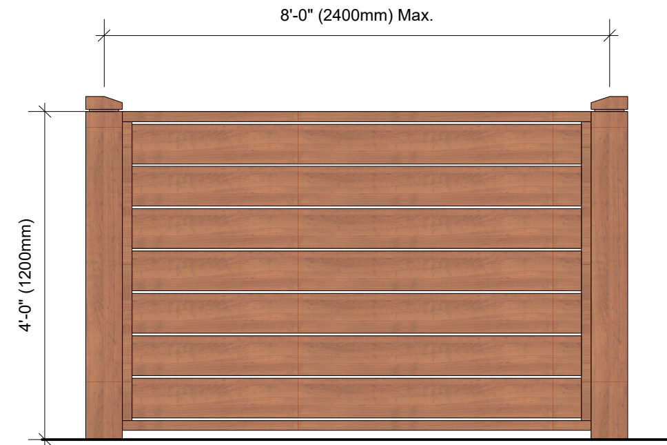
1.2m Ht. Cedar Fencing 1:20
