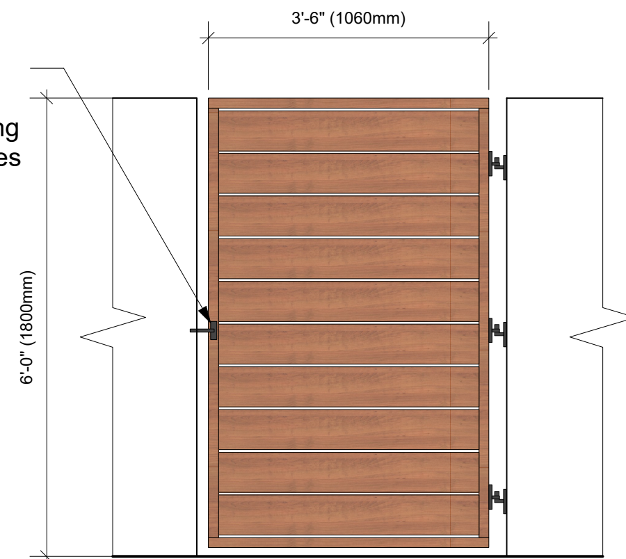
1.8m Ht. Cedar Gate 1:20
