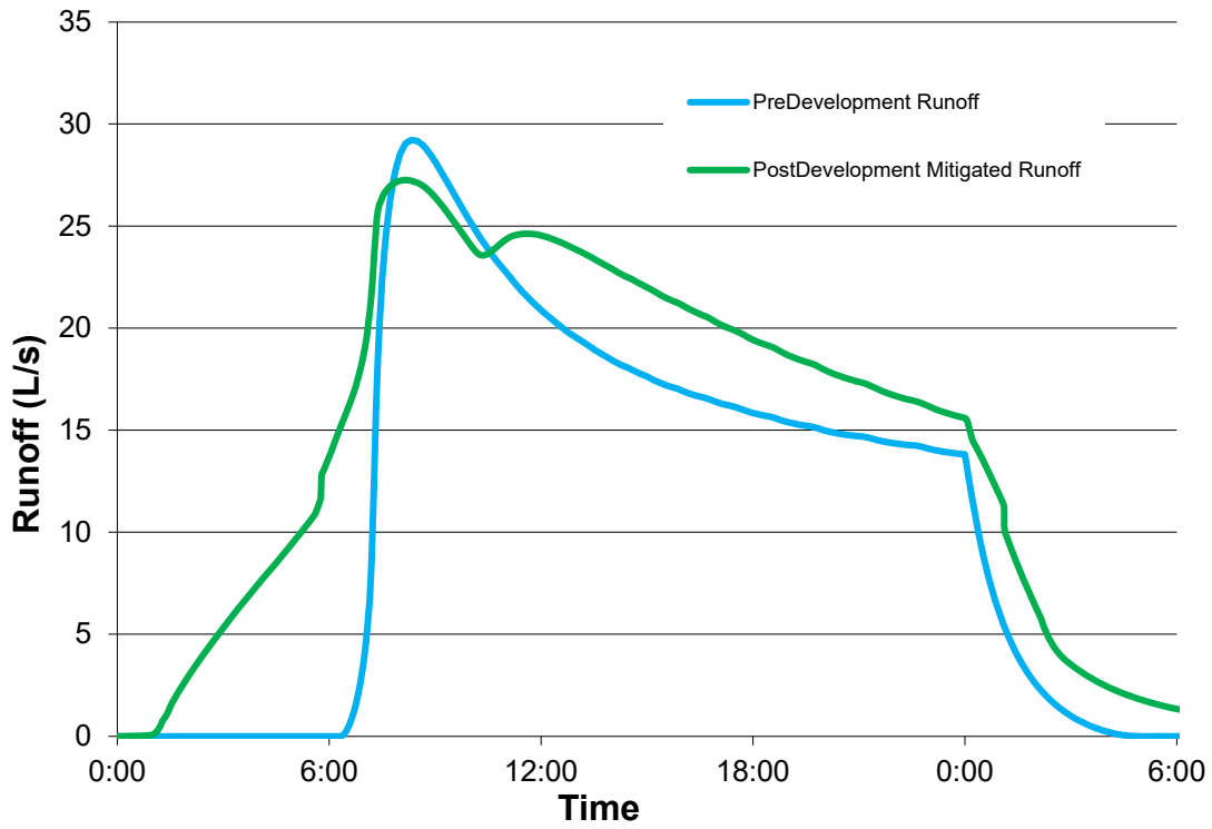
Figure 3: Runoff Hydrographs for the 2 year design rainfall event
