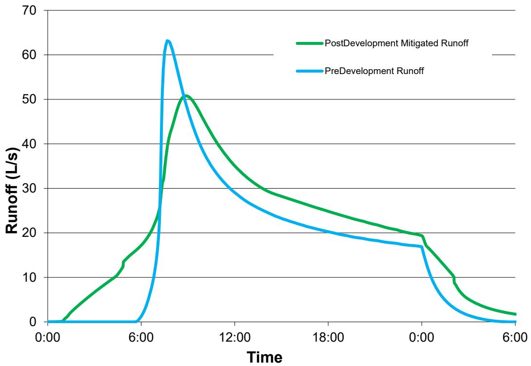
Figure 4: Runoff Hydrographs for the 5 year design rainfall event
