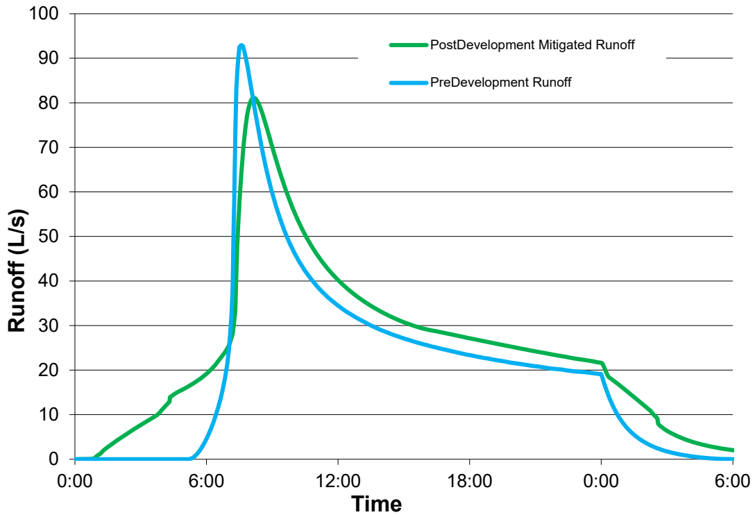
Figure 5: Runoff Hydrographs for the 10 year design rainfall event
