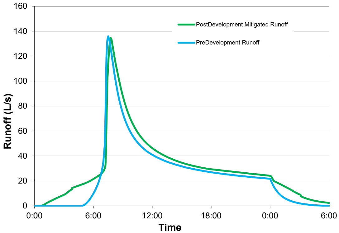
Figure 6: Runoff Hydrographs for the 25 year design rainfall event
