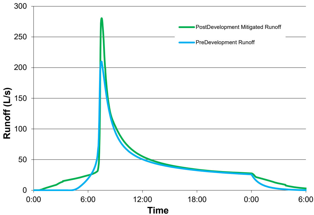
Figure 7: Runoff Hydrographs for the 100 year design rainfall event
