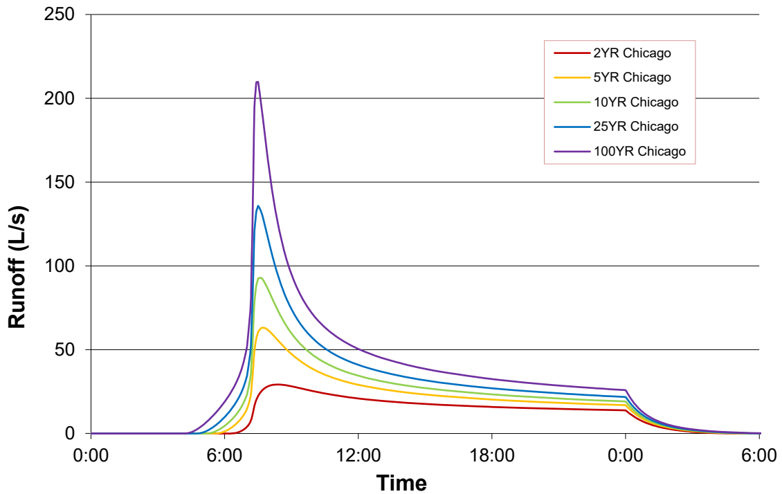
Figure 2: Runoff Hydrographs for the 2, 5, 10, 25 and 100-Year Design Storm Events under Existing Site Conditions
